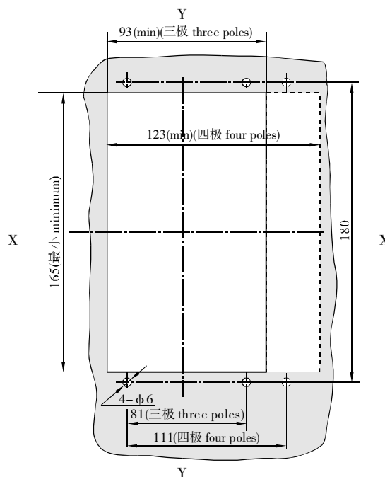
安装方式二开孔尺寸 Aperture Dimensions of the second mounting way
