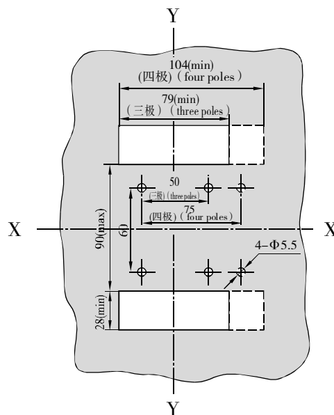
安装方式一开孔尺寸 Aperture Dimensions of the first mounting way
