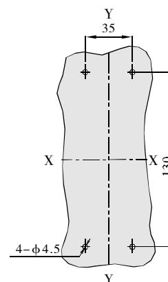
板前接线安装板开孔尺寸 Aperture Dimensions of the sub-panel, wiring on front of the board
