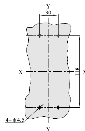
板前接线安装板开孔尺寸 Aperture Dimensions of the sub-panel, wiring in front of the board
